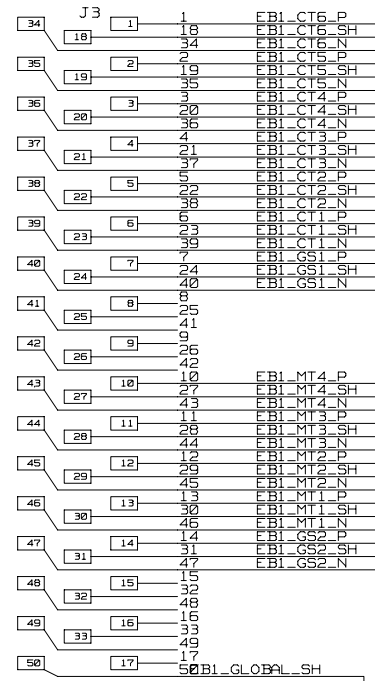
EXTENDED_BARREL CABLE_1 (EB1) SK-DIN41612-50 DSUB RT-ANG
