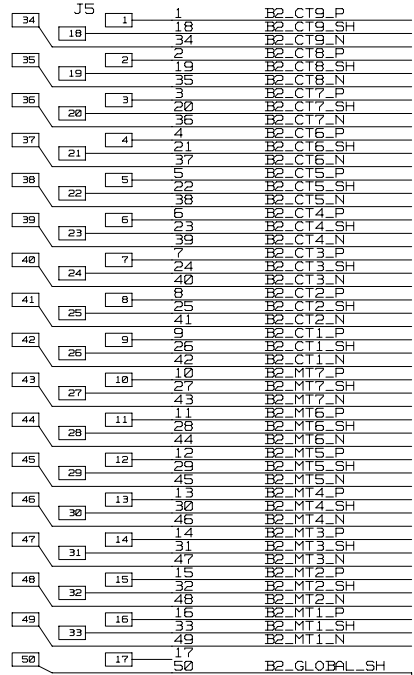
BARREL CABLE_2 (B2) SK-DIN41612-50 DSUB RT-ANG
