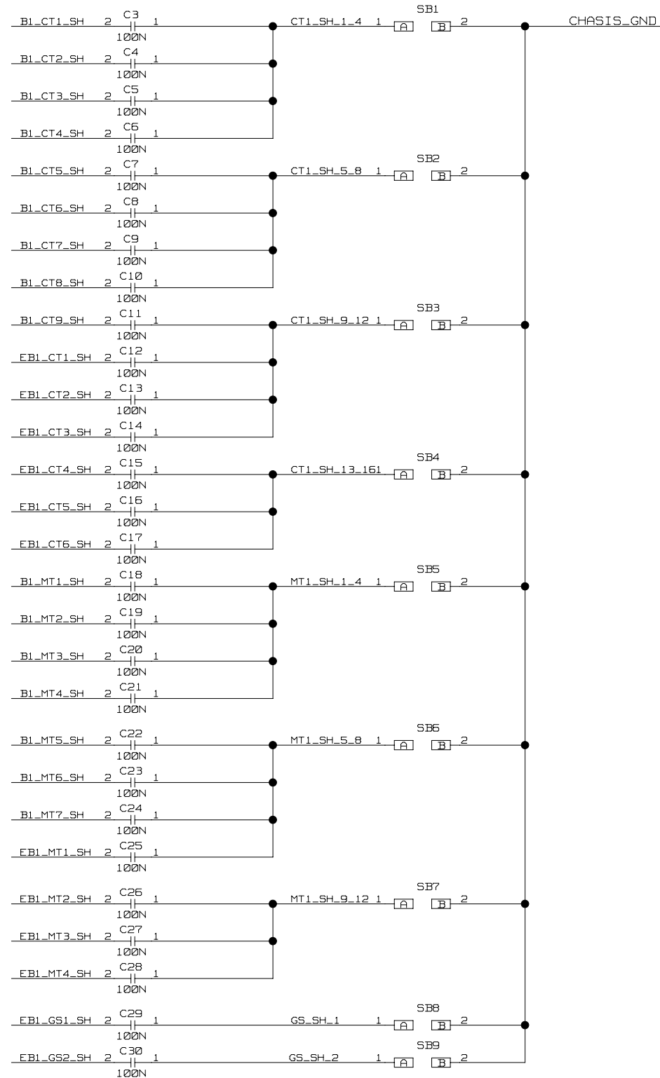
CALORIMETER_TRIGGER CABLE_1 (CT1) SK-DIN41612-37 DSUB RT-ANG
