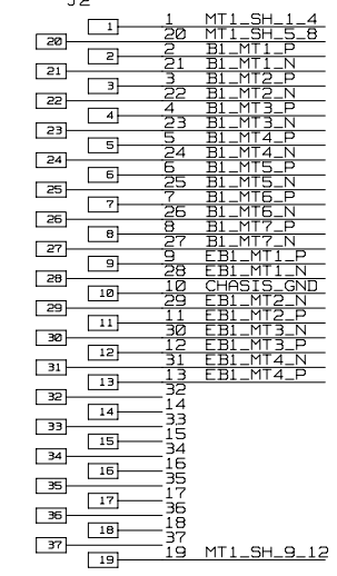
MUON_TRIGGER CABLE_1 (MT1) SK-DIN41612-37 DSUB RT-ANG
