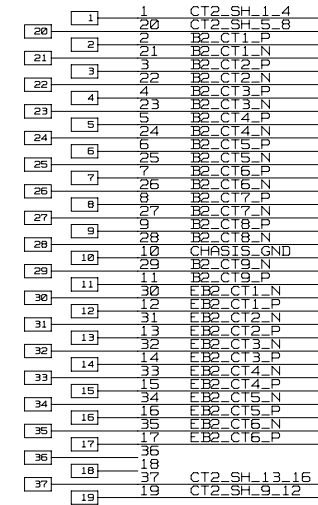
CALORIMETER_TRIGGER CABLE_2 (CT2) SK-DIN41612-37 DSUB RT-ANG
