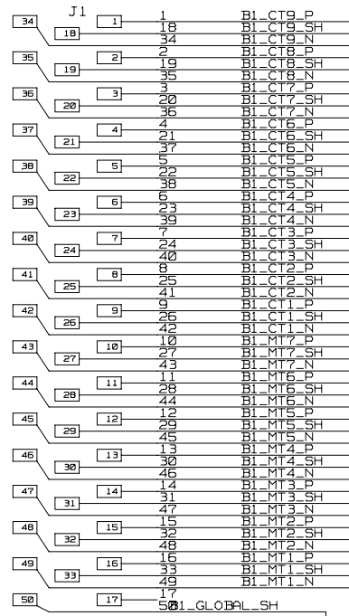
BARREL CABLE_1 (B1) SK-DIN41612-50 DSUB RT-ANG
