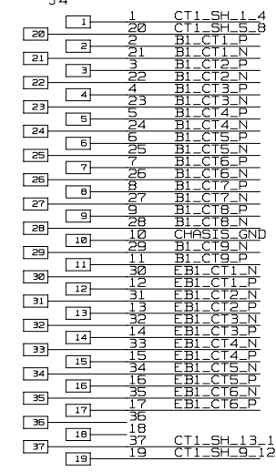
CALORIMETER_TRIGGER CABLE_1 (CT1) SK-DIN41612-37 DSUB RT-ANG
