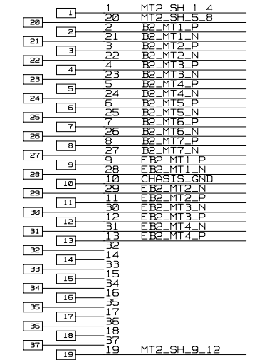
MUON_TRIGGER CABLE_2 (MT2) SK-DIN41612-37 DSUB RT-ANG
