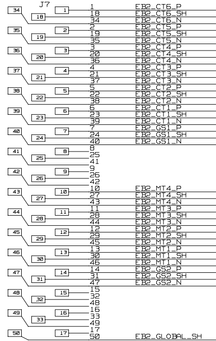
EXTENDED_BARREL CABLE_2 (EB2) SK-DIN41612-50 DSUB RT-ANG
