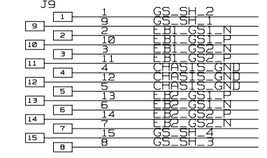
SK-DIN41612-15 DSUB RT-ANG
