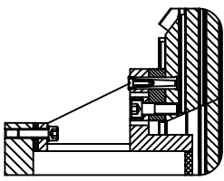
DETAIL J - SCALE 1:5 TYPICAL SECTION INTERFACE BETWEEN EE/HE AND BACKPLATE FIXTURE
