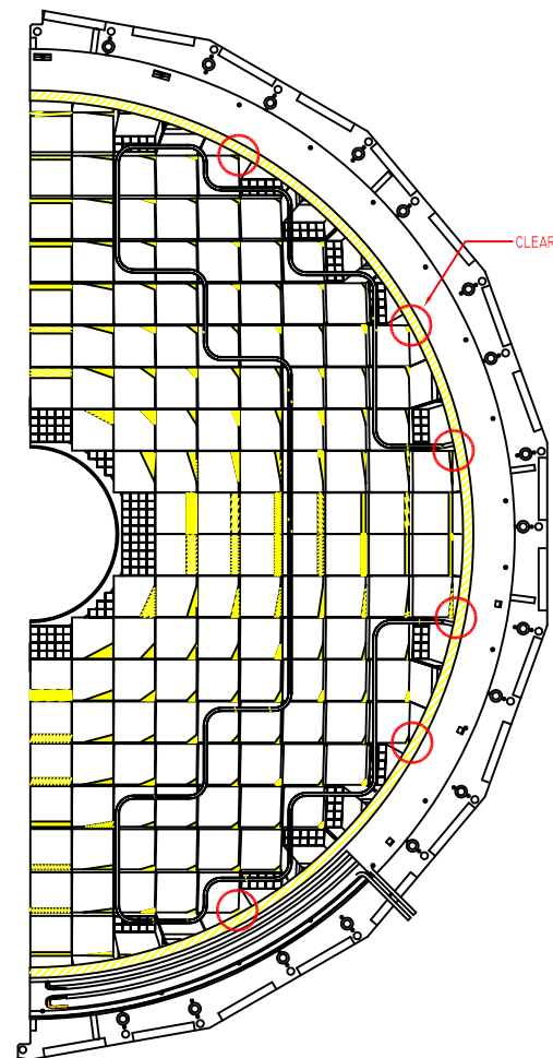
SECTION F-F
