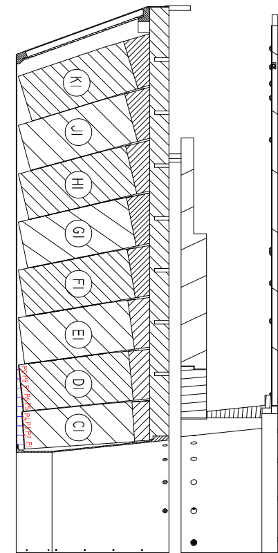
SECTION X-X
