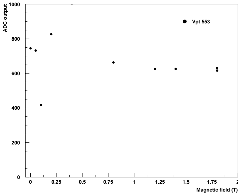
Figure 5. Examples of magnetic field scan on a typical VPT.
