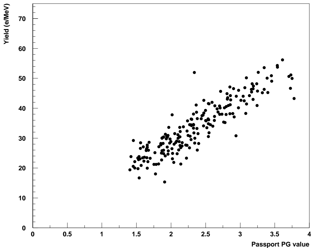
Figure 8. VPT response at 8^{\circ} - 25^{\circ} and 1.8T v quality factor PG
