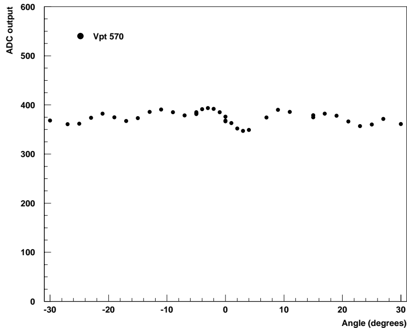
Figure 6. Angular scan at 1.8T on a typical VPT.
