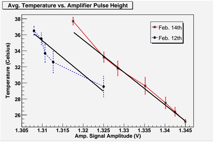
Fig 4: Amplifier fit
