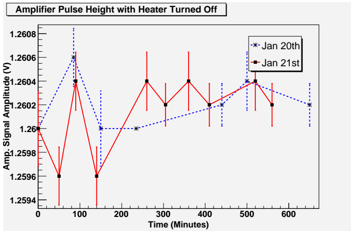
Fig 8: Amplifier stability
