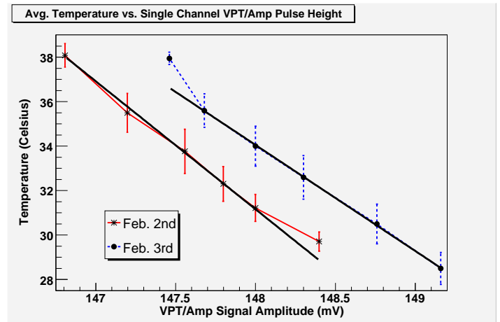
Fig 7: VPT/Amp fit
