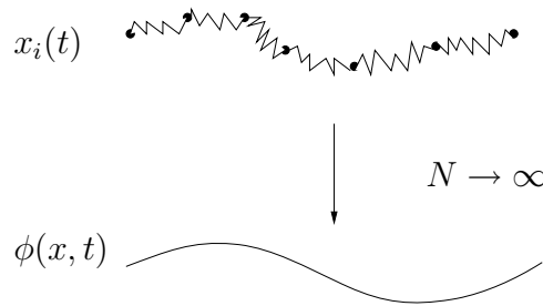
Figure 2: From N coupled point masses to a continuous string, i.e. infinitely many degrees of freedom.
